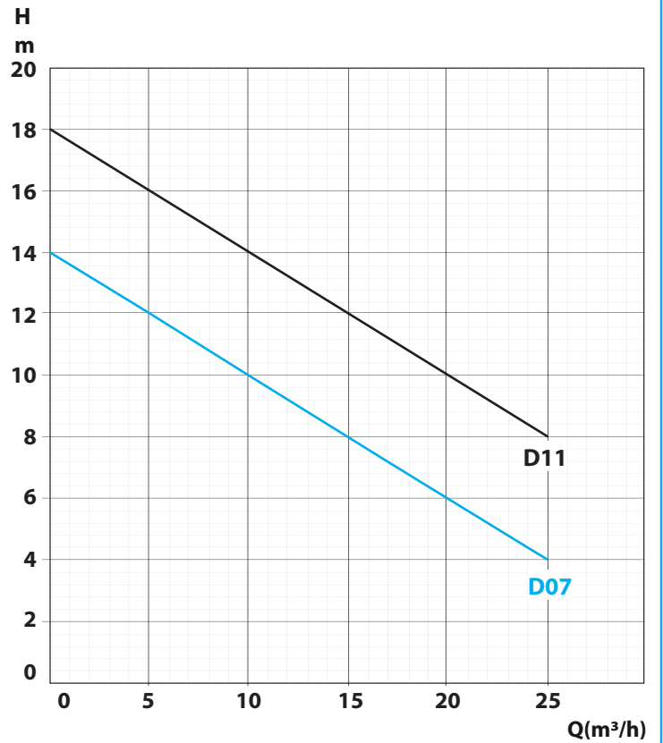
SCV Pump Performance Curve
