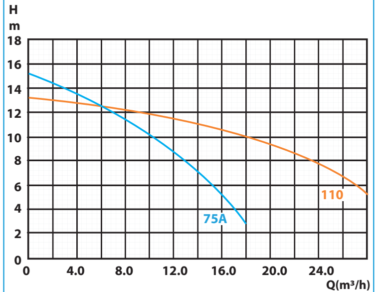
SWVS Pump Performance Curve
