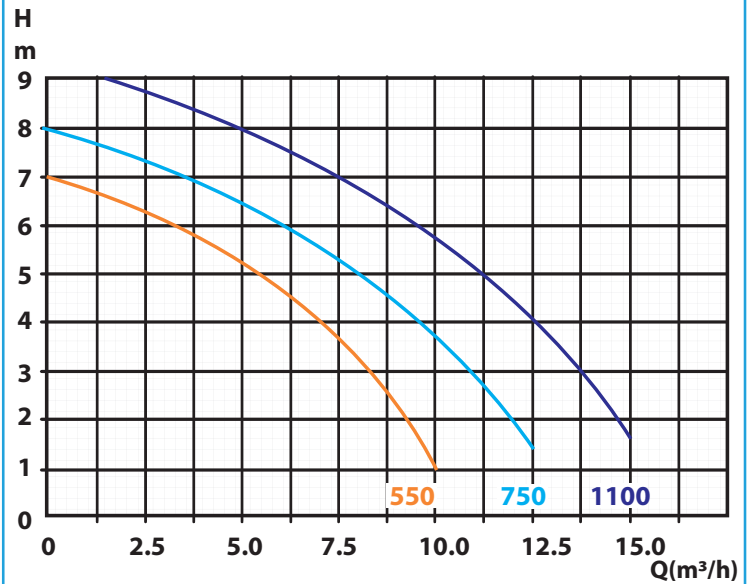
SGW Pump Performance Curve
