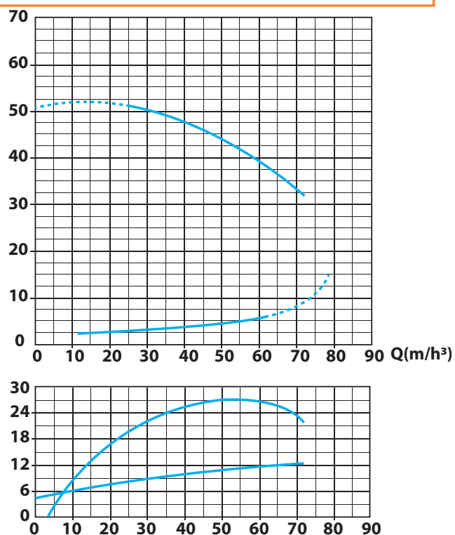
SEN 50-200B Pump Performance Curve
