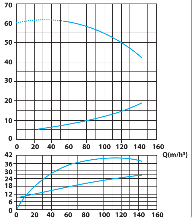
SEN 65-200A Pump Performance Curve
