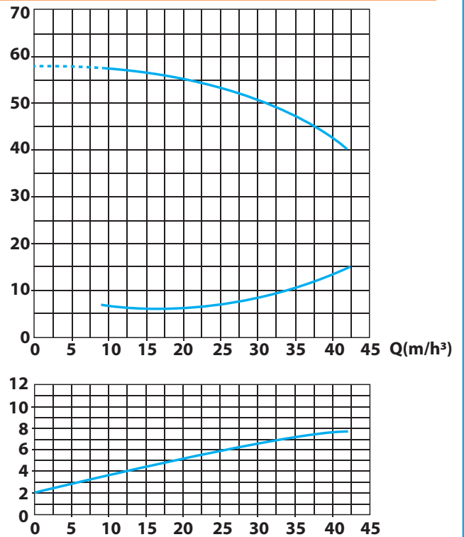
SEN 40-200A Pump Performance Curve
