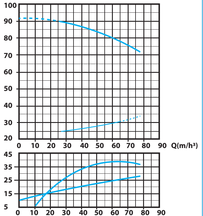
SEN 50-250A Pump Performance Curve
