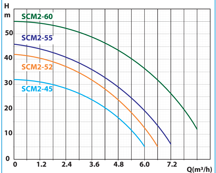
SCM2 Pump Performance Curve
