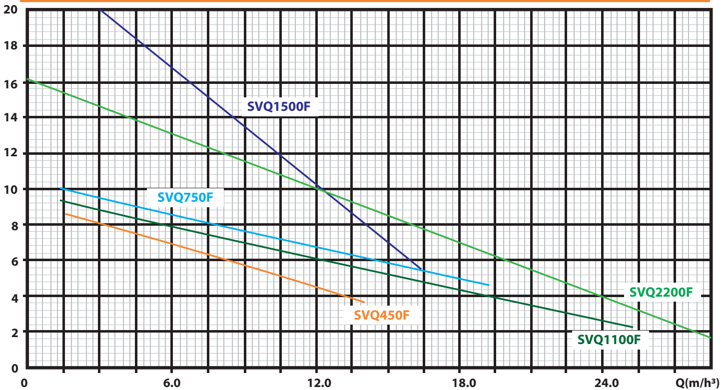
SVQ Pump Performance Curve
